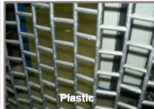
Two 1200mm screens – three grades – up to 20tph
