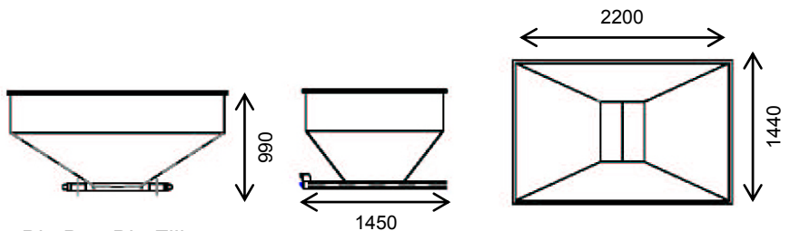
Big Bag Bin Filler
