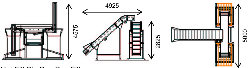
Uni-Fill Big Bag Box Filler
