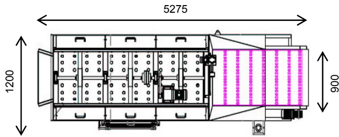
Model 1030 vee tank
