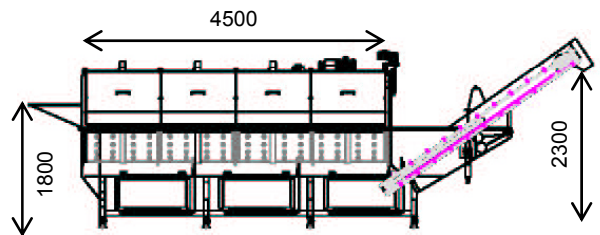
Model 1245 with horizontal floor tank
