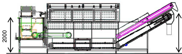
Tumblers destoner – model 1230 washer with scraper chain sludge removal – water filter elevator
