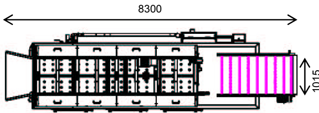
Model 1245 with horizontal floor tank
