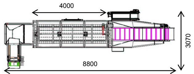
Tumblers destoner – model 1230 washer with scraper chain sludge removal – water filter elevator
